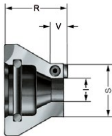
A14 Driving discs, with interchangeable carbide driving plates 6 x 3.2, right-hand rotation, max. workpiece hardness 40 HRC
