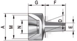
A06 Interchangeable inserts B for centerless workpieces 60°
