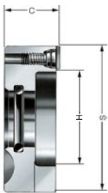
A14 Driving discs, with interchangeable carbide driving plates 9.5 x 3.2, left-hand rotation, max. workpiece hardness 40 HRC
