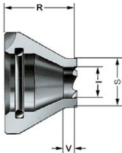
A14 Driving discs, toothed, right- and left-hand rotation, max. workpiece hardness 35 HRC
