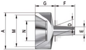
A06 Interchangeable inserts A for centerless workpieces 60°
