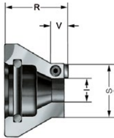
A14 Driving discs, with interchangeable carbide driving plates 6 x 3.2, right- and left-hand rotation, max. workpiece hardness 40 HRC
