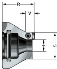
A14 Driving discs, with interchangeable carbide driving plates 6 x 3.2, left-hand rotation, max. workpiece hardness 40 HRC
