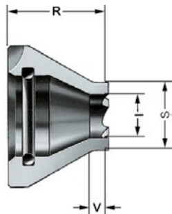
A14 Driving discs, toothed, left-hand rotation, max. workpiece hardness 35 HRC
