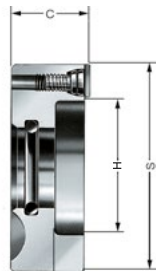
A14 Driving discs, with interchangeable carbide driving plates 9.5 x 3.2, right-hand rotation, max. workpiece hardness 40 HRC
