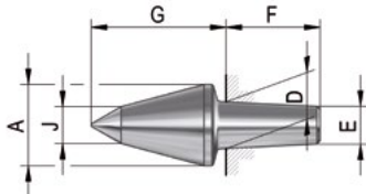
A06 Interchangeable inserts for tubular workpieces 60°
