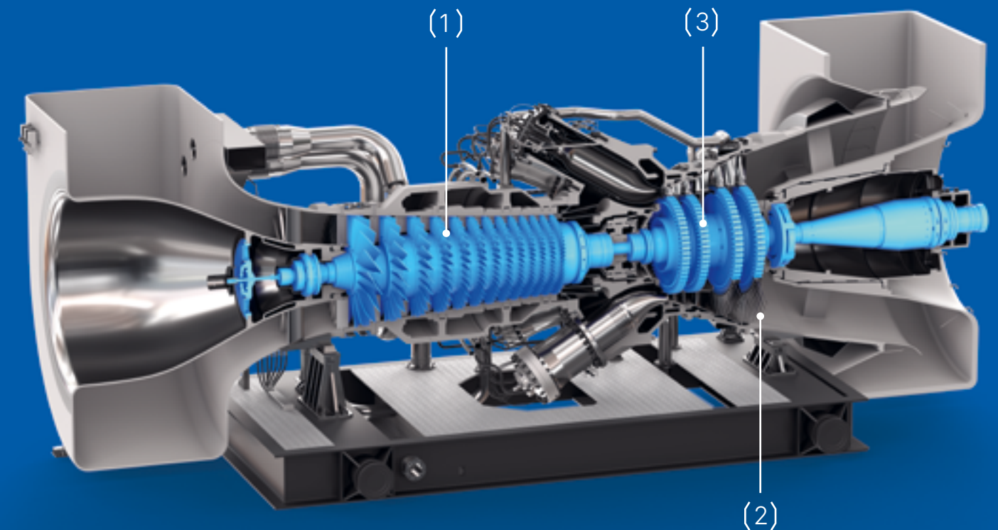
Gas turbine
