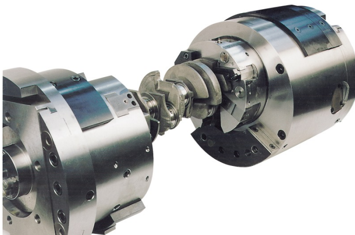
Award for a technically sophisticated product from Röhme: the HTF cycle chuck
