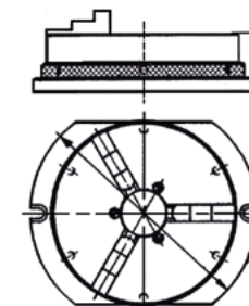
Dimensions KRF, cylindrical centre mount
