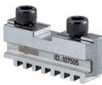
A09 Base jaw GB, DIN 6350, with fixing screw
