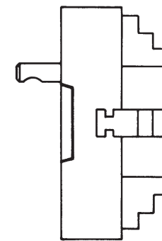
A26 ISO 702-2 (DIN 55029), ASA B 5.9, type D, with studs for Camlock
