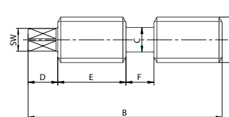
Adjusting spindle
