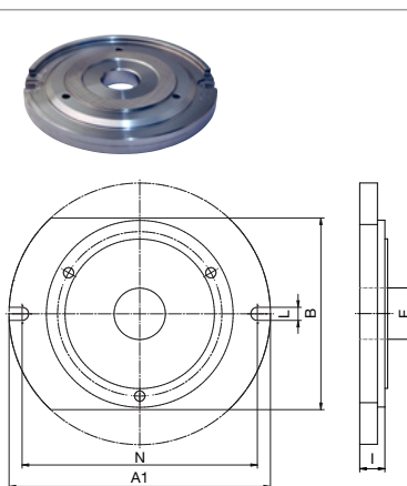
A09 Base plates for lathe chucks with cylindrical centre mount, DIN 6350
