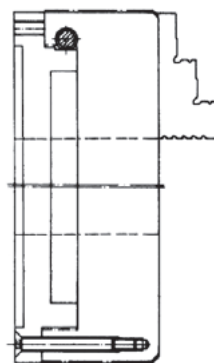
A09 ZS Hi-Tru, with one set outward stepped jaws and one set inward stepped jaws, DIN 6350, cylindrical centre mount, form A
