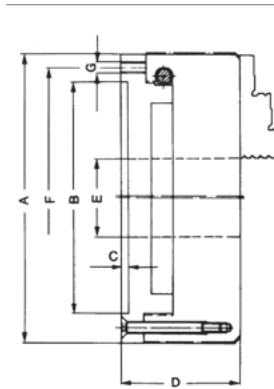
Dimensions ZS Hi-Tru, DIN 6350, cylindrical centre mount, Form A
