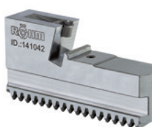
C 21 Draw-down jaws, additional clamping range, for interchangeable clamping inserts, diagonally toothing, 1 piece, without clamping inserts
