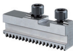
A28 Base jaw GB, 3-jaw set, diagonally toothing, with mounting bolts
