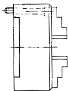
Tool group A09 Geared scroll chucks ZG-ZGU mounting from front; cylindrical centre mount
